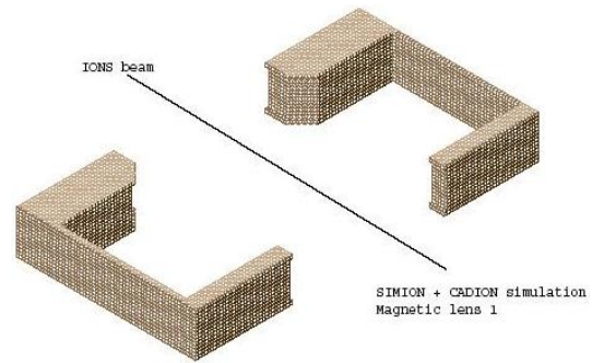
Fig. (8) The optimized pole piece profile of magnetic lens obtained by SIMION 7
