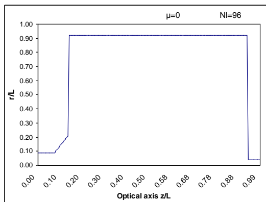
Fig. (7) A two dimension profile of a pole piece for a magnetic lens with \mu=0 and NI = 96 ampere-turns
