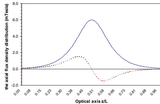
Fig. (4) The optimum axial magnetic flux density distribution B(z) with its first derivative obtained by the dynamic programming procedure and artificial intelligence technique
