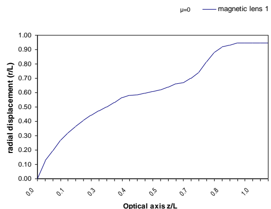
Fig. (5) The ion beam trajectories of magnetic lens under infinite magnification condition (for a constant length L=20 mm)
