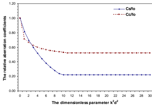
Fig. (6) The relative spherical and chromatic aberration coefficients of the optimized magnetic lens related to the dimensionless parameter k^2d^2
